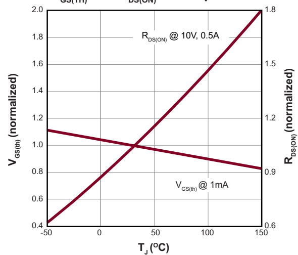
V GS(TH) and R DS(ON) w/ Temperature
